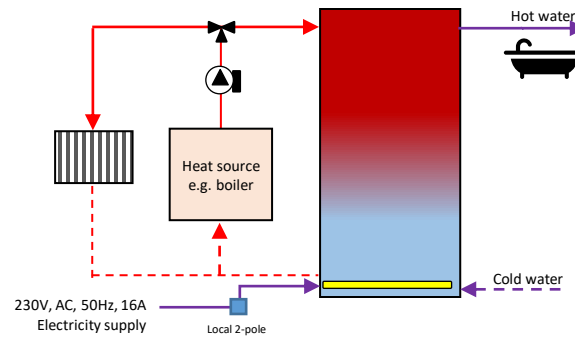
UniQ HW X heated by external heat source and with standby electric heater
