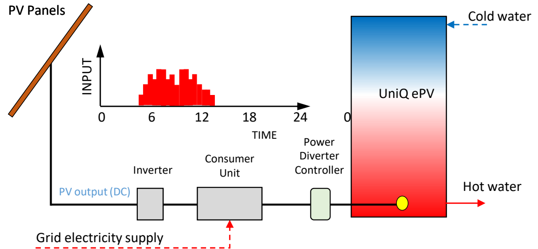
UniQ eHW X battery heated by grid electricity and solar PV
